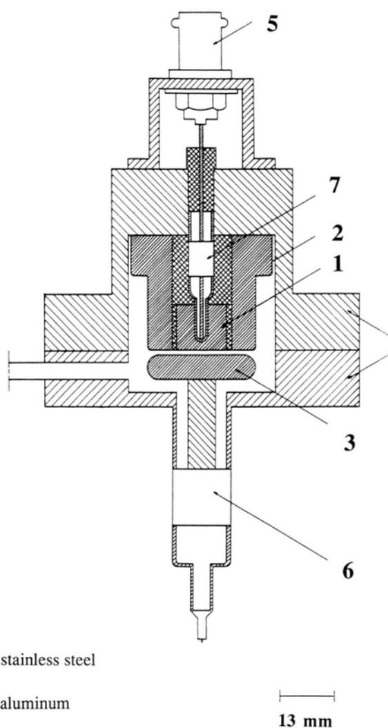
Fig. 1. Schematic drawing of the conductivity cell; 1 measurement electrode; 2 guard ring electrode; 3 high voltage electrode; 4 UHV-flange; 5 BNC jack; 6 high voltage feed through; 7 feedthrough.
